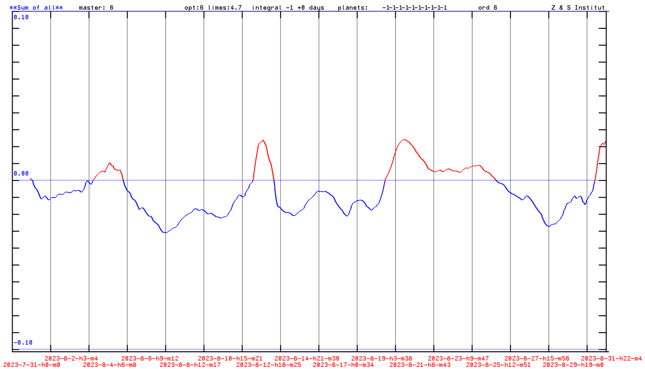
Figure 7: Curve of pattern A for the period 2023-8. Above the center line, the probability of a pattern A earthquake is greater.
