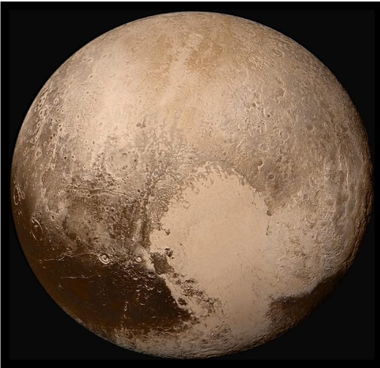
Figure 10: image of Pluto (Wikipedia).
