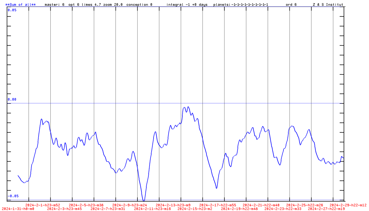
Fig. 8: Curve of pattern A for the period 2024-02. Above the center line, the probability of a pattern A earthquake is greater.
