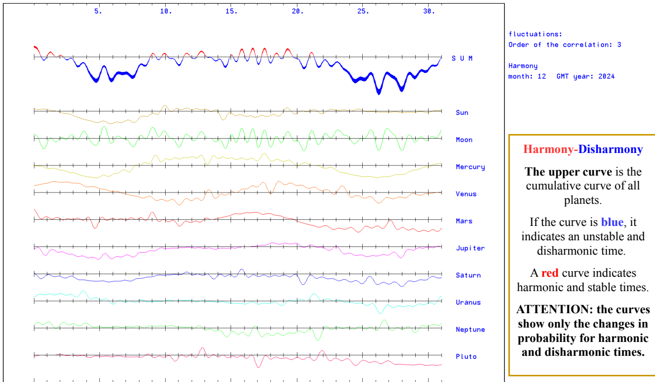
Fig. 1: The quality of time in December 2024; full moon is on December 15, new moon on December 1.
