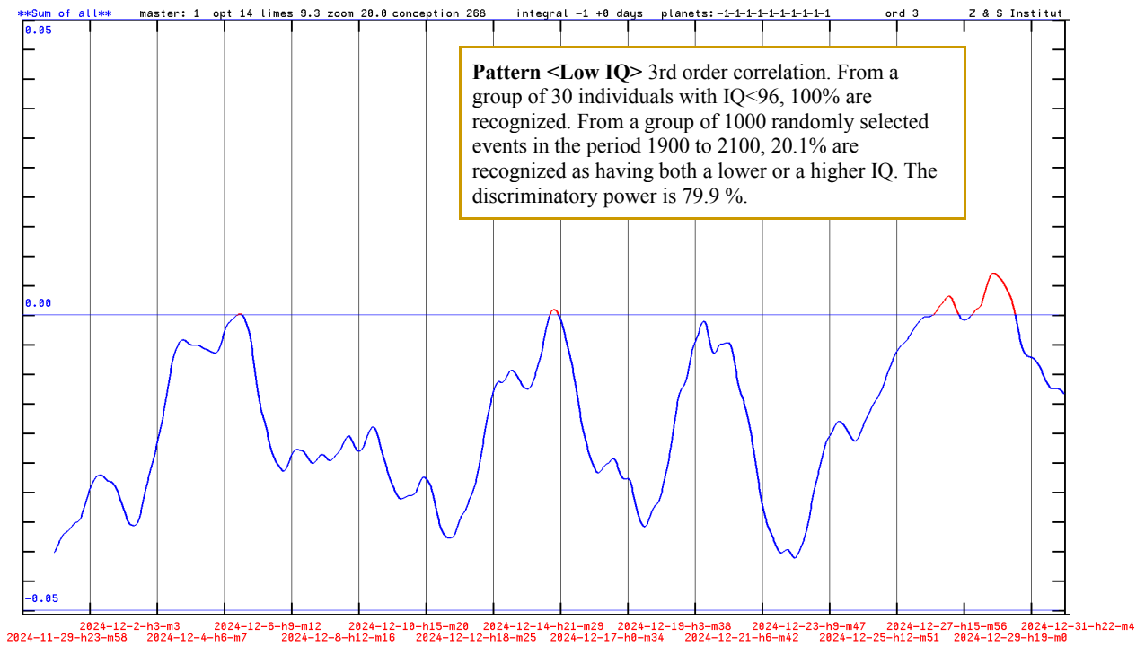
Fig. 11: The probability of a lower IQ at conception of an intended pregnancy in December 2024. If the curve is above the center line (red part of the curve), then this time falls into the "Low IQ" pattern. The birth is 8 months and 24 days later than December 2024).
