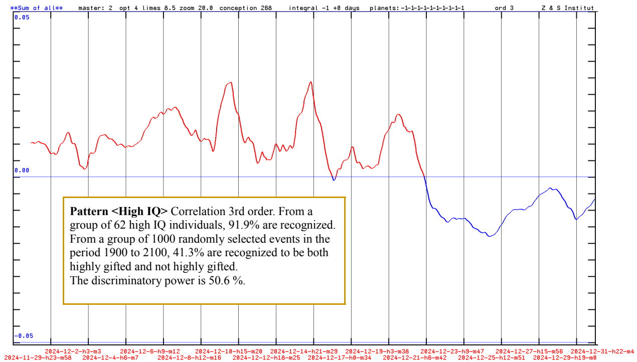
Fig. 10: The probability of a higher IQ at conception of an intended pregnancy in December 2024. If the curve is above the center line (red part of the curve), then this time falls into the "High IQ" pattern for high achievers. The birth takes place 8 months and 24 days later than December 2024.
