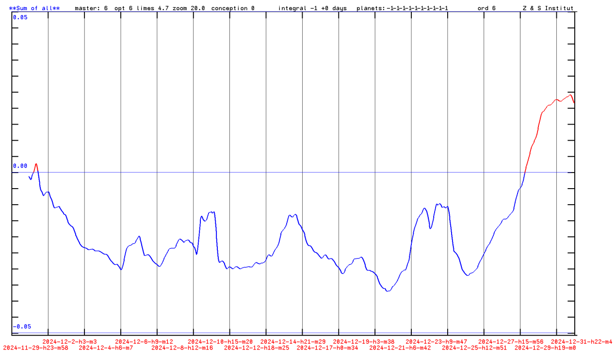
Fig. 8: Curve of pattern A for the period 2024-12. Above the center line, the probability of a pattern A earthquake is greater.
