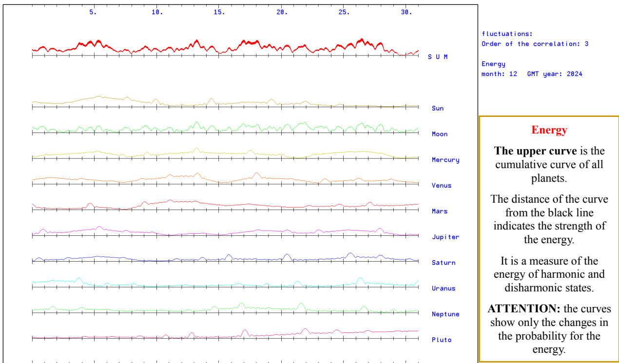
Fig. 3: The energy of the quality of time in December 2024
