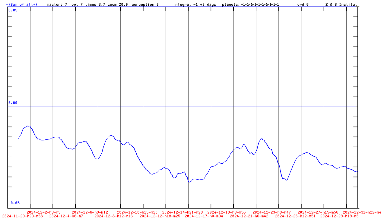
Fig. 9: Curve of pattern B. 513 earthquakes for the period 2024-12. Above the center line, the probability of a pattern A earthquake is greater.
