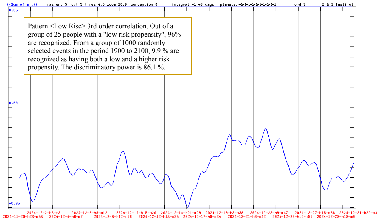
Fig. 7: The probability for the characteristic "low risk appetite/strong need for harmony" when a person is born in December 2024. If the curve is above the center line, then this time falls into the pattern for a "low risk appetite/strong need for harmony"
