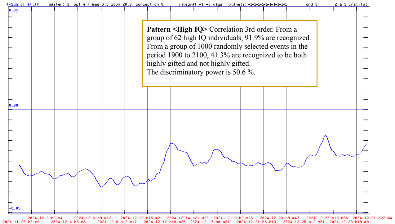
Fig. 5: The probability of a higher IQ at birth in December 2024. If the curve is above the center line, then this time falls into the "High IQ" pattern for gifted people.
