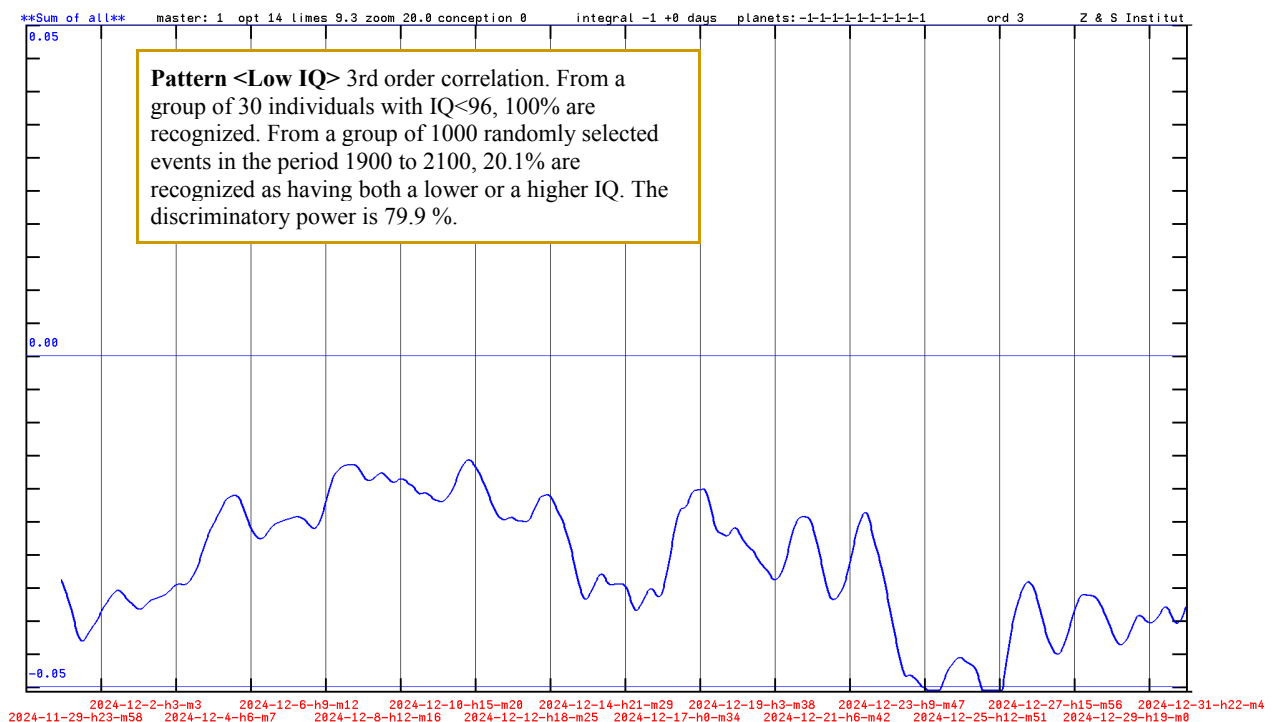
Fig. 6: The probability of a low IQ at birth in December 2024. If the curve is above the center line, then this time falls within the pattern for a low IQ.
